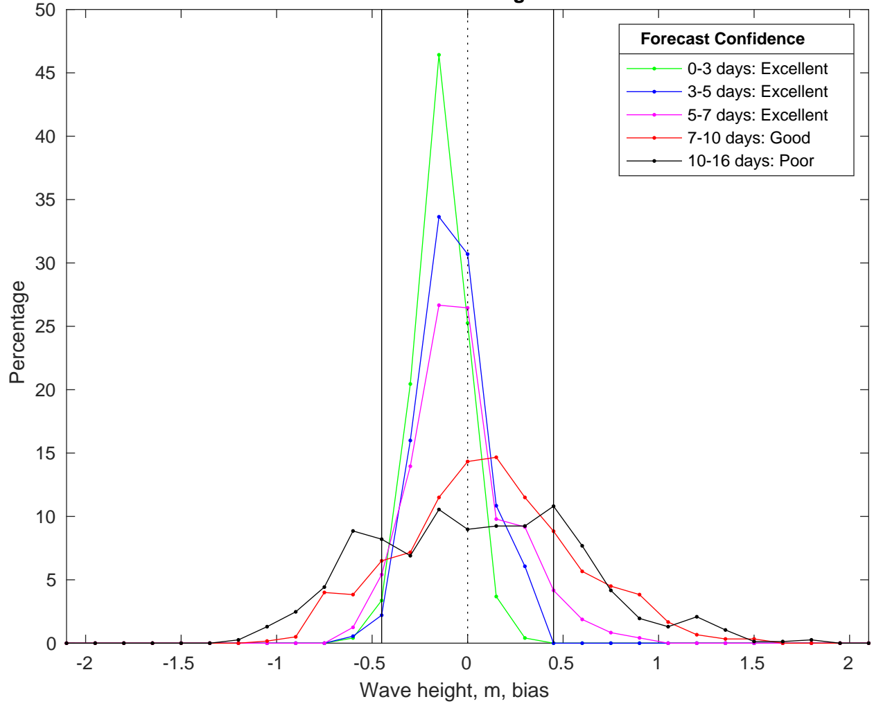
NDBC 41040 vs GFS Waves Bias Histogram: 25-Mar-2025
