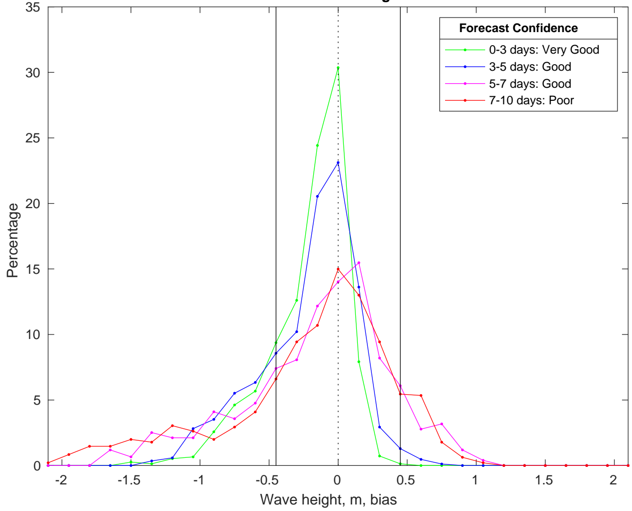
NDBC 42019 vs CMEMS Waves Bias Histogram: 25-Mar-2025
