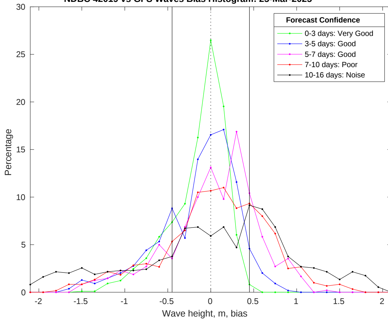
NDBC 42019 vs GFS Waves Bias Histogram: 25-Mar-2025
