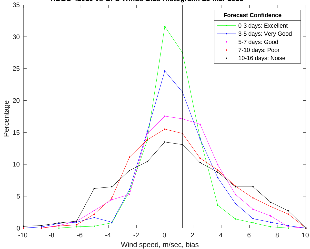
NDBC 42019 vs GFS Winds Bias Histogram: 25-Mar-2025
