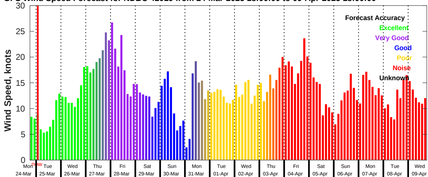
GFS Wind Speed Forecast for NDBC 42019 from 24-Mar-2025 18:00:00 to 09-Apr-2025 18:00:00
