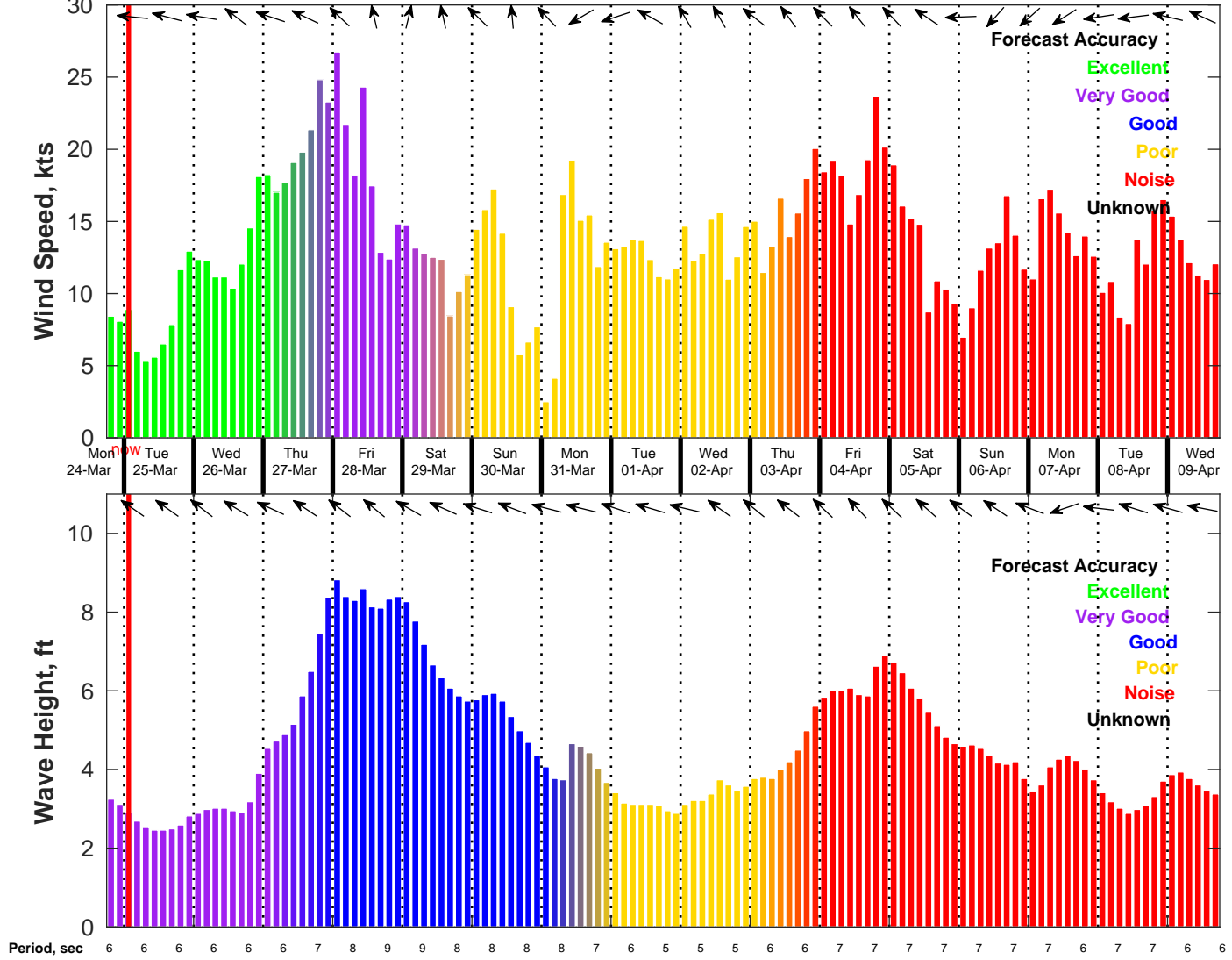
Wind & Wave Forecast for NDBC 42019 from 24-Mar-2025 18:00:00 to 09-Apr-2025 18:00:00
