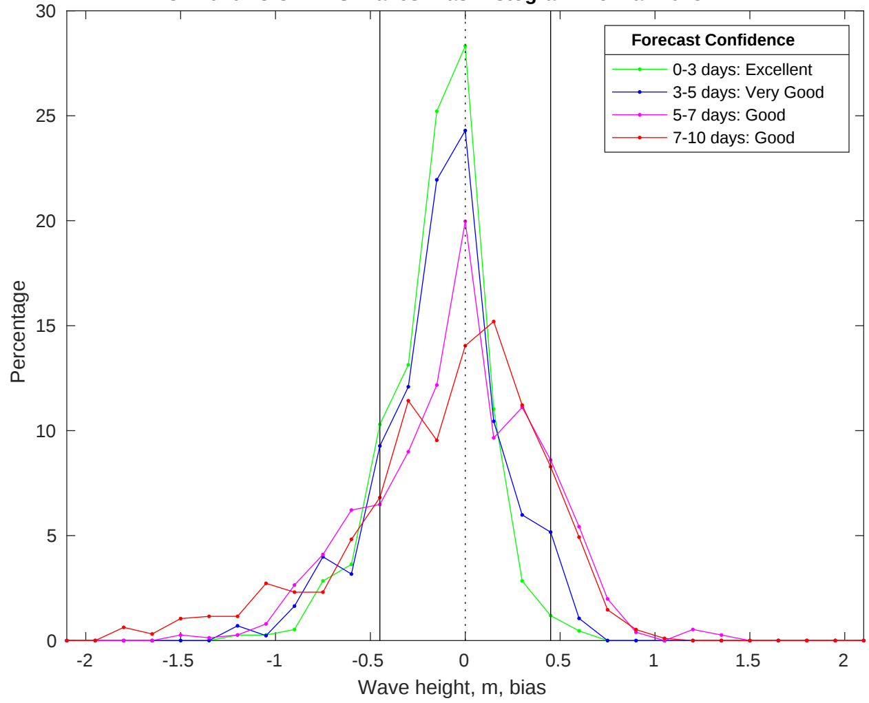
NDBC 42020 vs CMEMS Waves Bias Histogram: 25-Mar-2025
