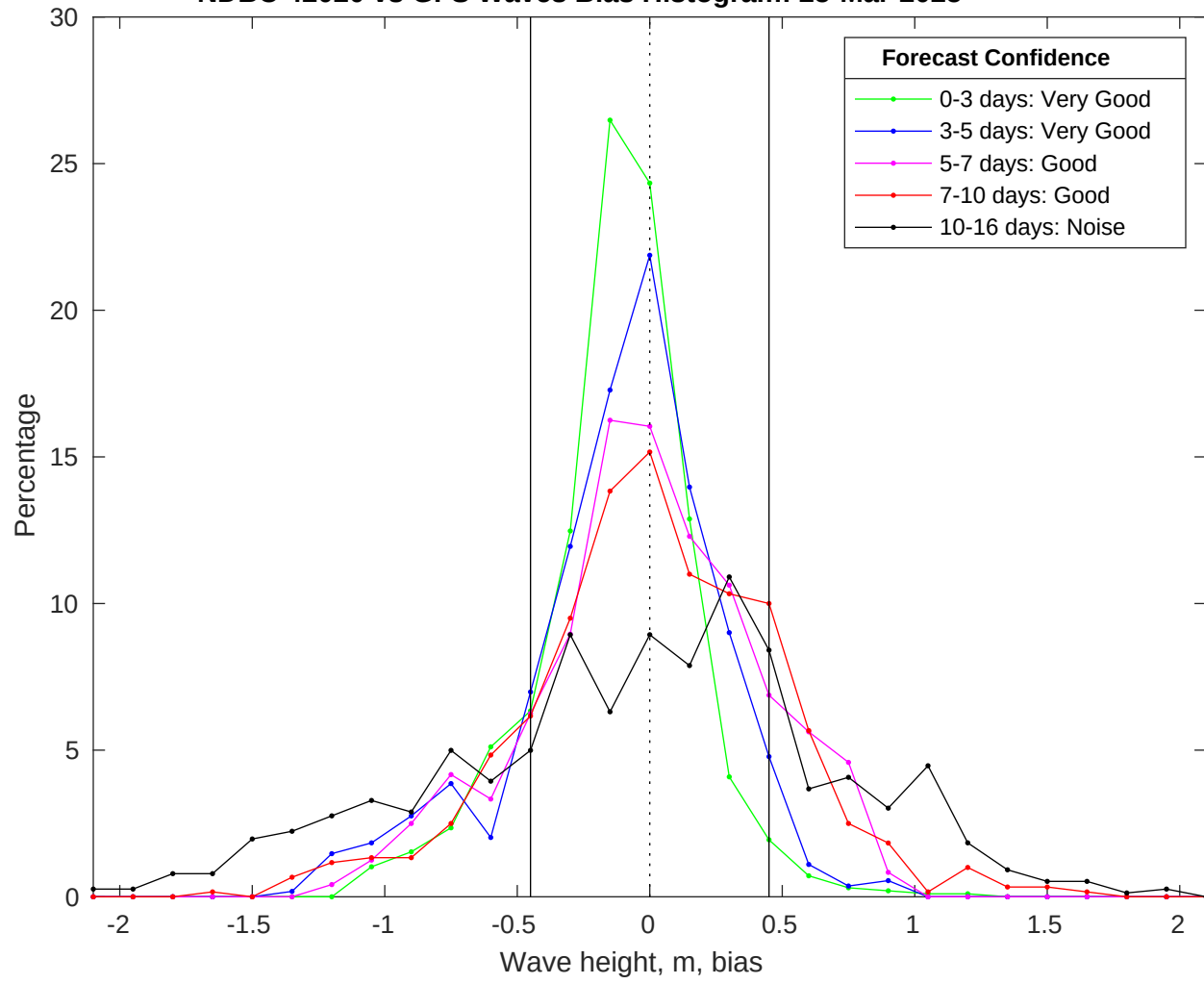
NDBC 42020 vs GFS Waves Bias Histogram: 25-Mar-2025
