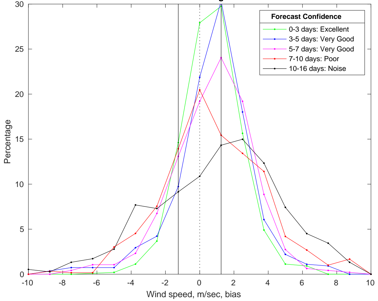
NDBC 42020 vs GFS Winds Bias Histogram: 25-Mar-2025
