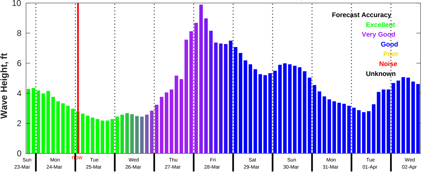
CMEMS Wave Forecast for NDBC 42020 from 23-Mar-2025 18:00:00 to 02-Apr-2025 18:00:00
