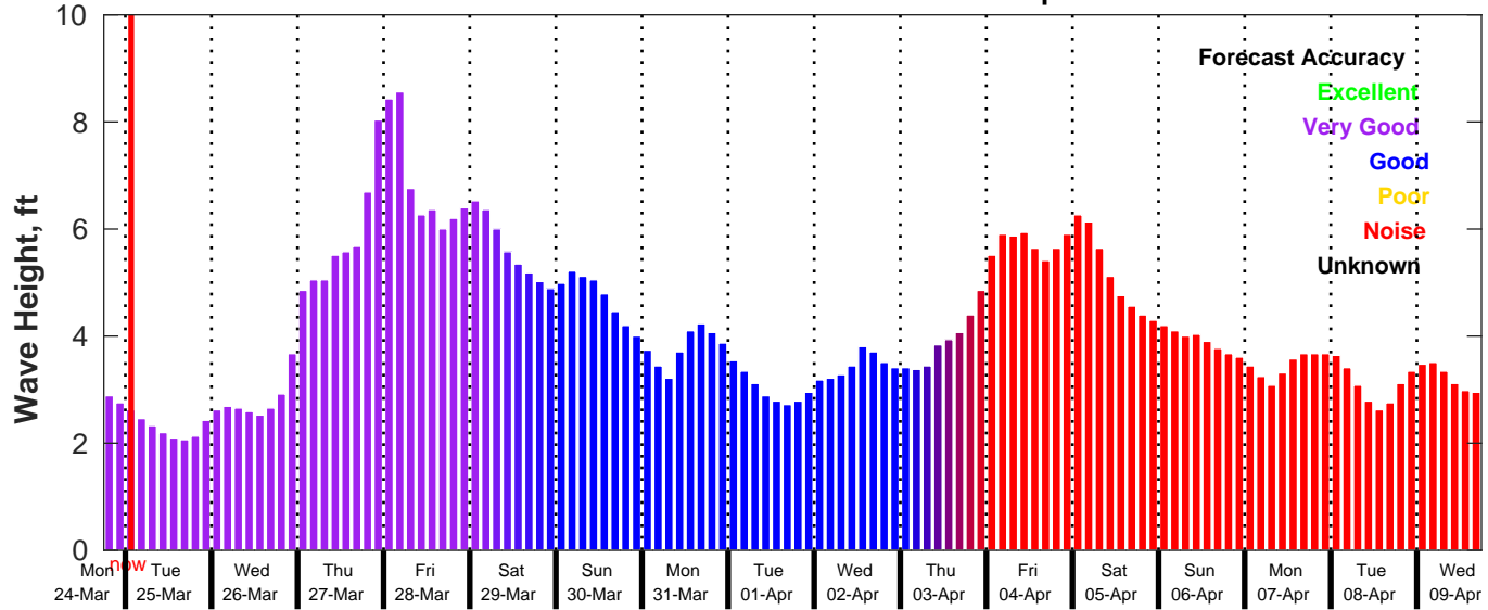
GFS Wave Forecast for NDBC 42020 from 24-Mar-2025 18:00:00 to 09-Apr-2025 18:00:00
