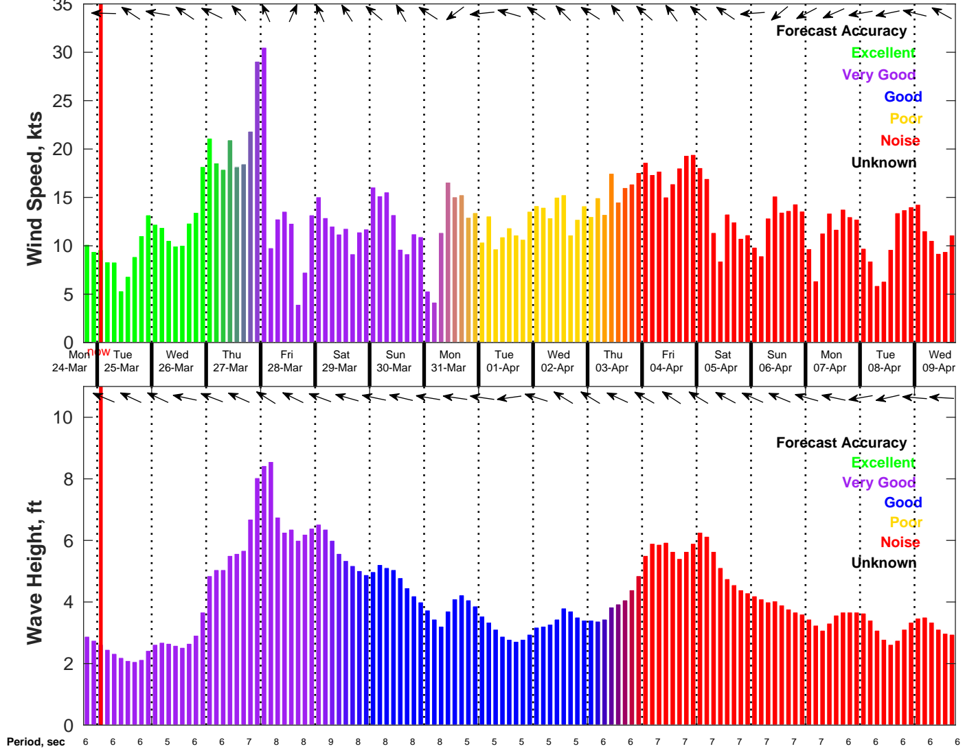
Wind & Wave Forecast for NDBC 42020 from 24-Mar-2025 18:00:00 to 09-Apr-2025 18:00:00
