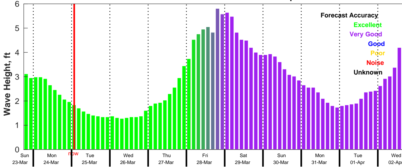
CMEMS Wave Forecast for NDBC 42035 from 23-Mar-2025 18:00:00 to 02-Apr-2025 18:00:00
