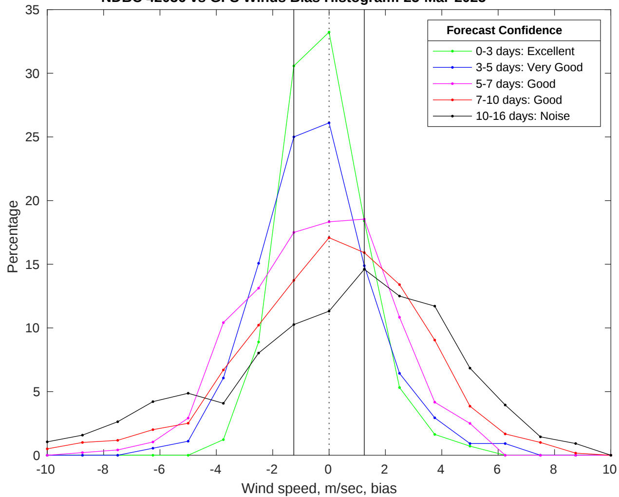
NDBC 42036 vs GFS Winds Bias Histogram: 25-Mar-2025
