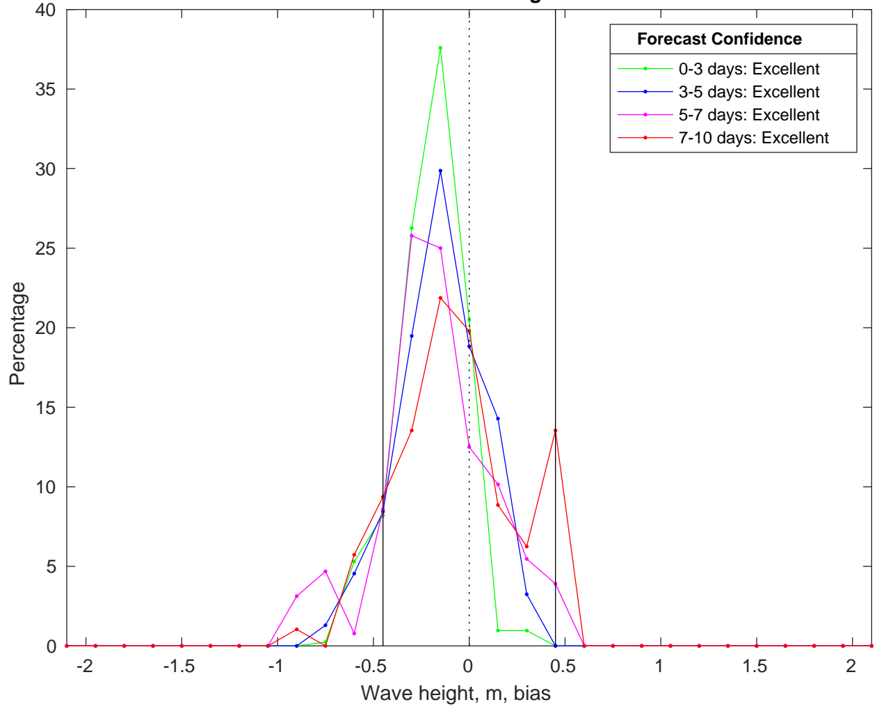
NDBC 42040 vs CMEMS Waves Bias Histogram: 25-Mar-2025
