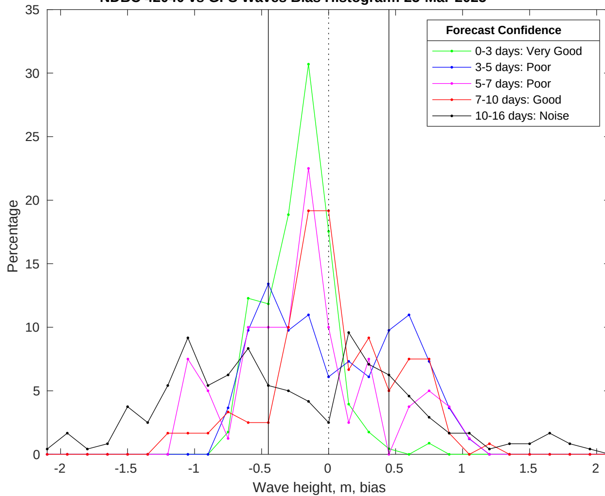
NDBC 42040 vs GFS Waves Bias Histogram: 25-Mar-2025
