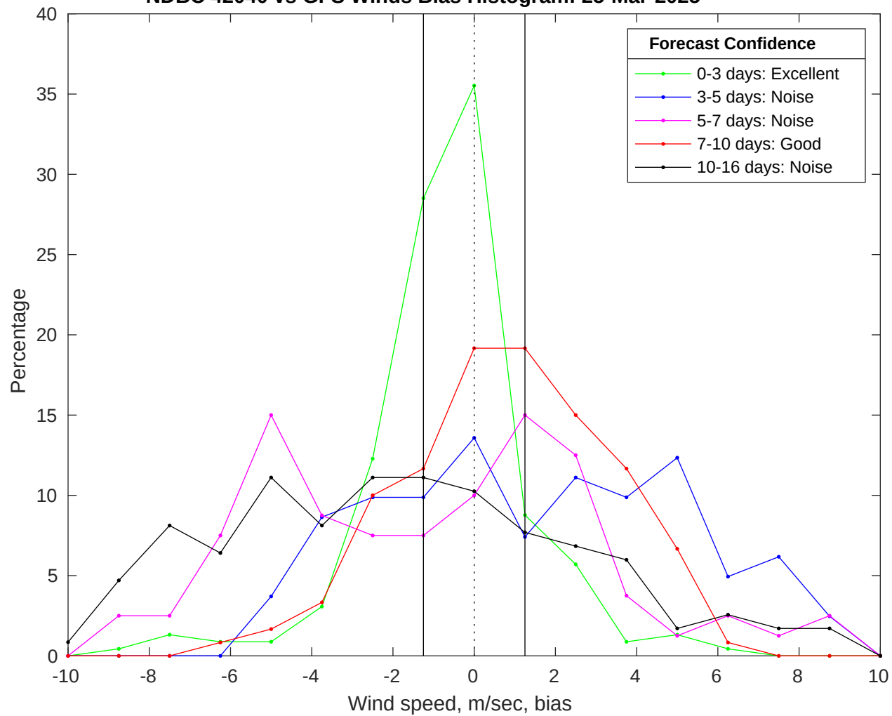
NDBC 42040 vs GFS Winds Bias Histogram: 25-Mar-2025
