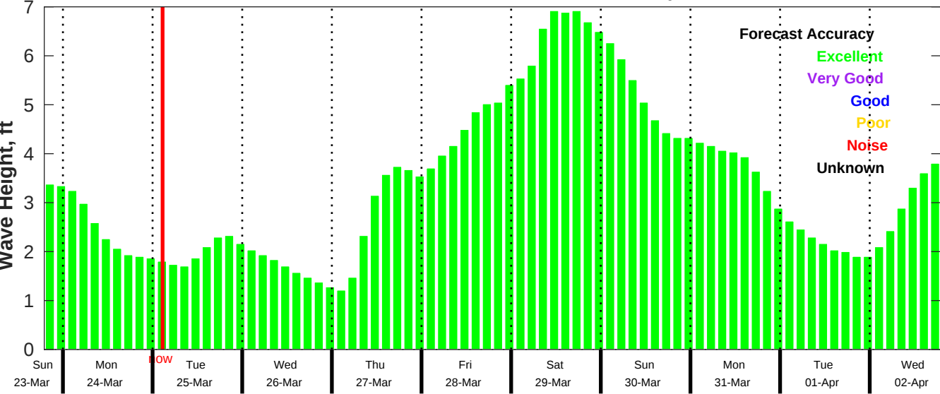
CMEMS Wave Forecast for NDBC 42040 from 23-Mar-2025 19:00:00 to 02-Apr-2025 19:00:00
