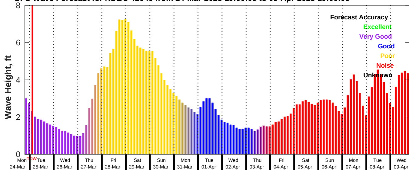
GFS Wave Forecast for NDBC 42040 from 24-Mar-2025 19:00:00 to 09-Apr-2025 19:00:00
