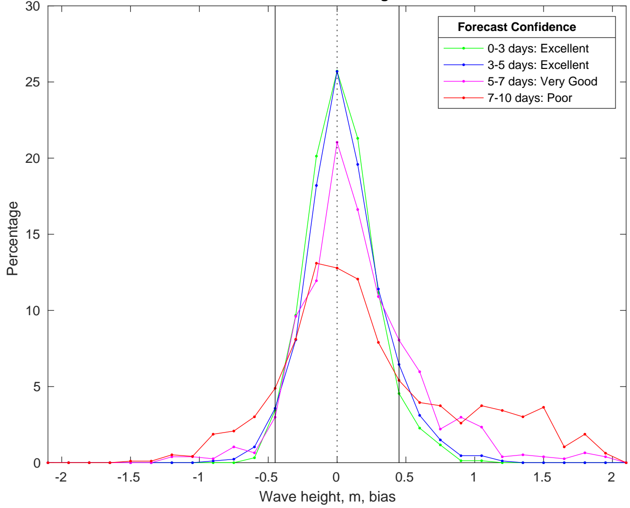
NDBC 46011 vs CMEMS Waves Bias Histogram: 25-Mar-2025
