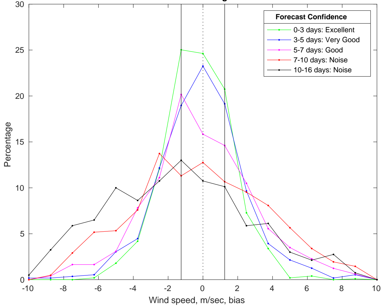
NDBC 46011 vs GFS Winds Bias Histogram: 25-Mar-2025
