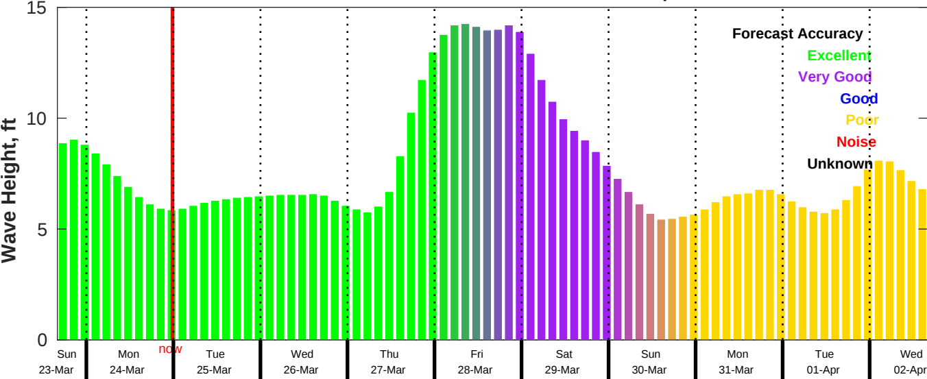
CMEMS Wave Forecast for NDBC 46011 from 23-Mar-2025 16:00:00 to 02-Apr-2025 16:00:00
