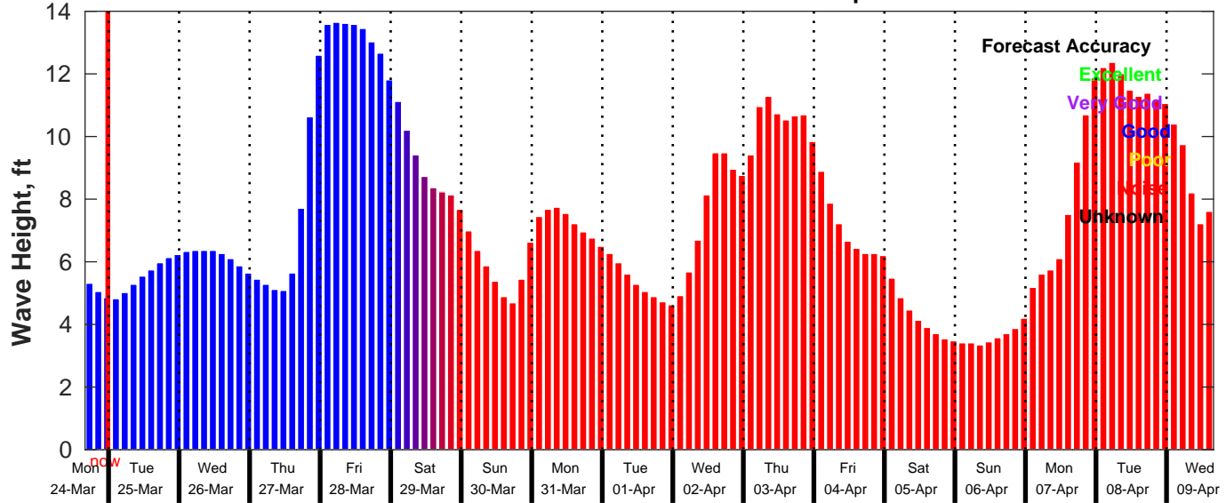
GFS Wave Forecast for NDBC 46011 from 24-Mar-2025 16:00:00 to 09-Apr-2025 16:00:00
