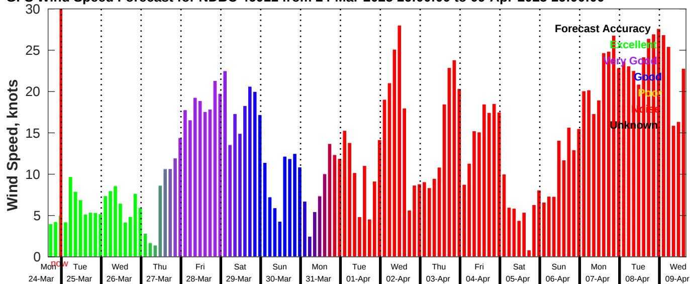
GFS Wind Speed Forecast for NDBC 46011 from 24-Mar-2025 16:00:00 to 09-Apr-2025 16:00:00
