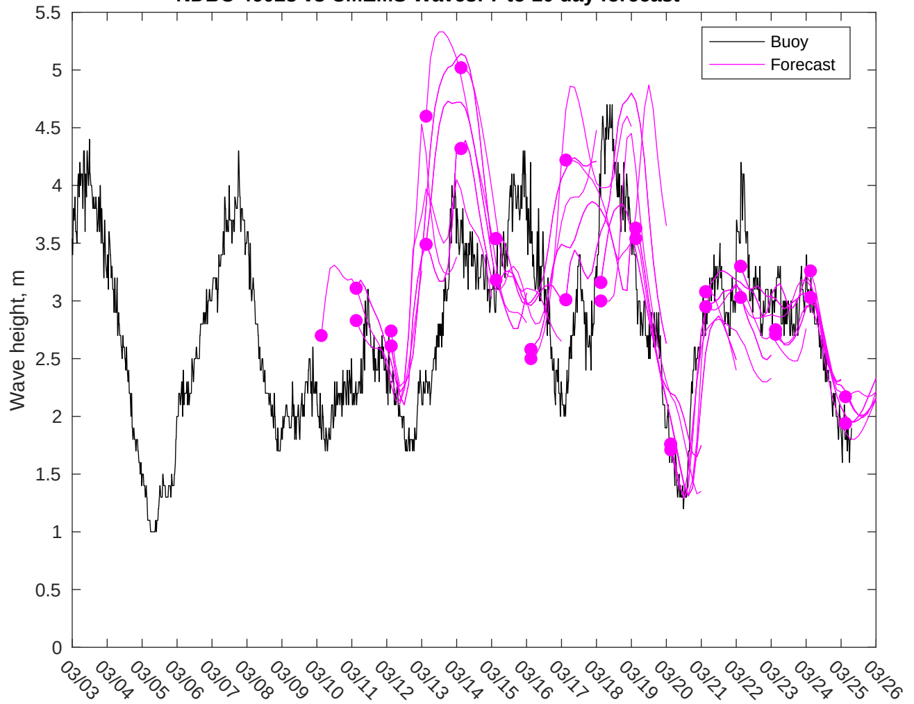
NDBC 46028 vs CMEMS Waves: 7 to 10 day forecast
