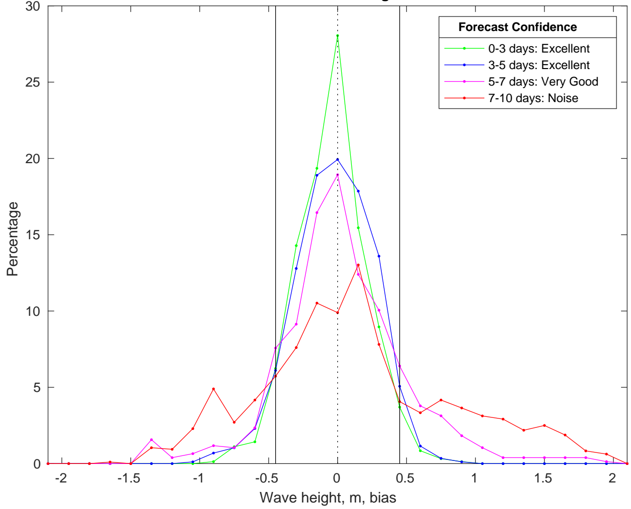
NDBC 46028 vs CMEMS Waves Bias Histogram: 25-Mar-2025
