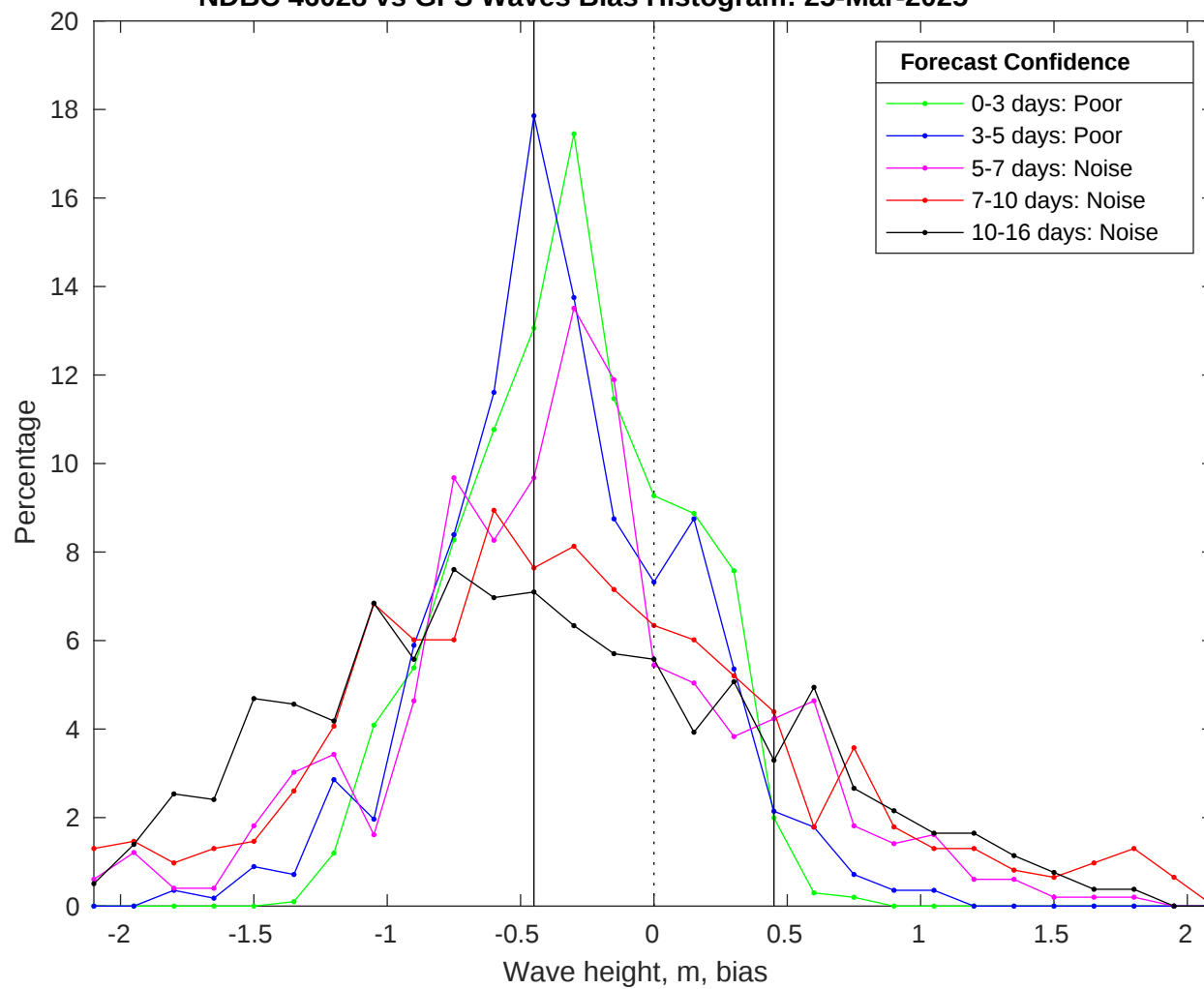
NDBC 46028 vs GFS Waves Bias Histogram: 25-Mar-2025
