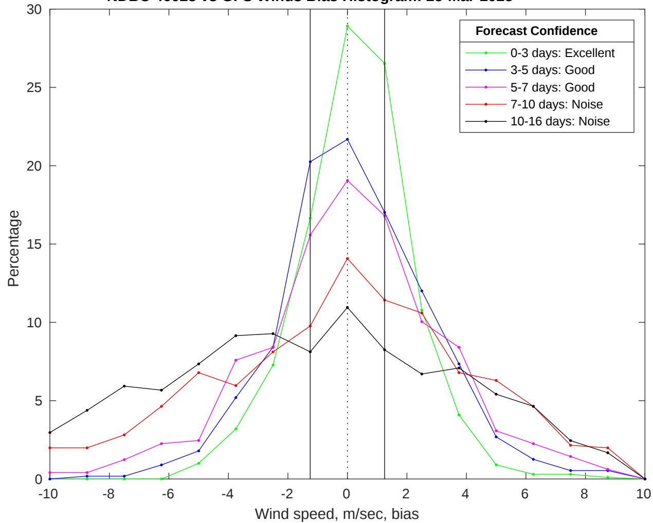
NDBC 46028 vs GFS Winds Bias Histogram: 25-Mar-2025
