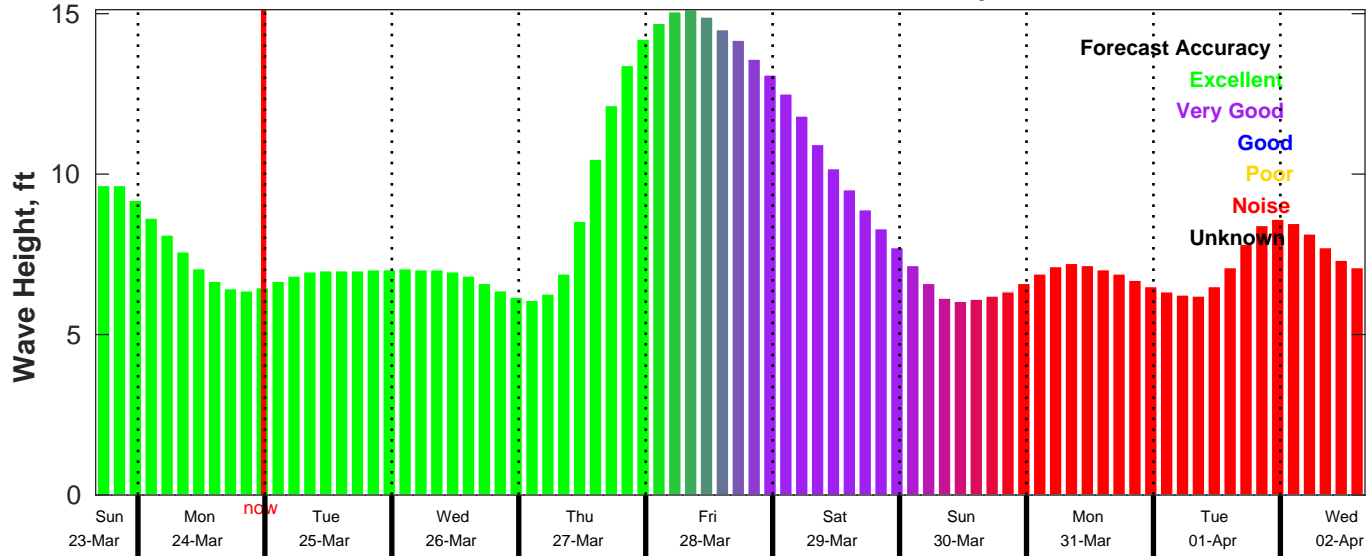
CMEMS Wave Forecast for NDBC 46028 from 23-Mar-2025 16:00:00 to 02-Apr-2025 16:00:00
