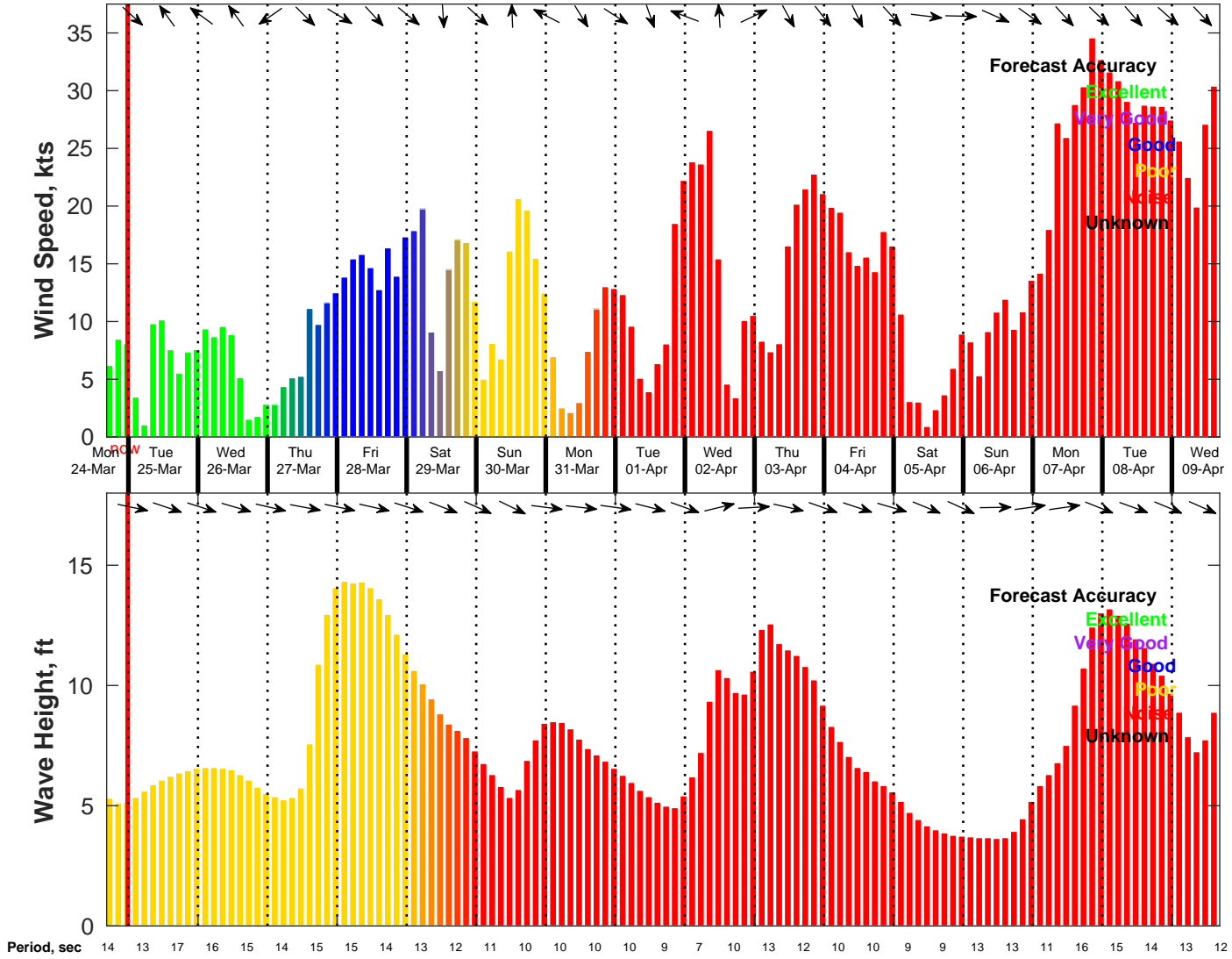
Wind & Wave Forecast for NDBC 46028 from 24-Mar-2025 16:00:00 to 09-Apr-2025 16:00:00
