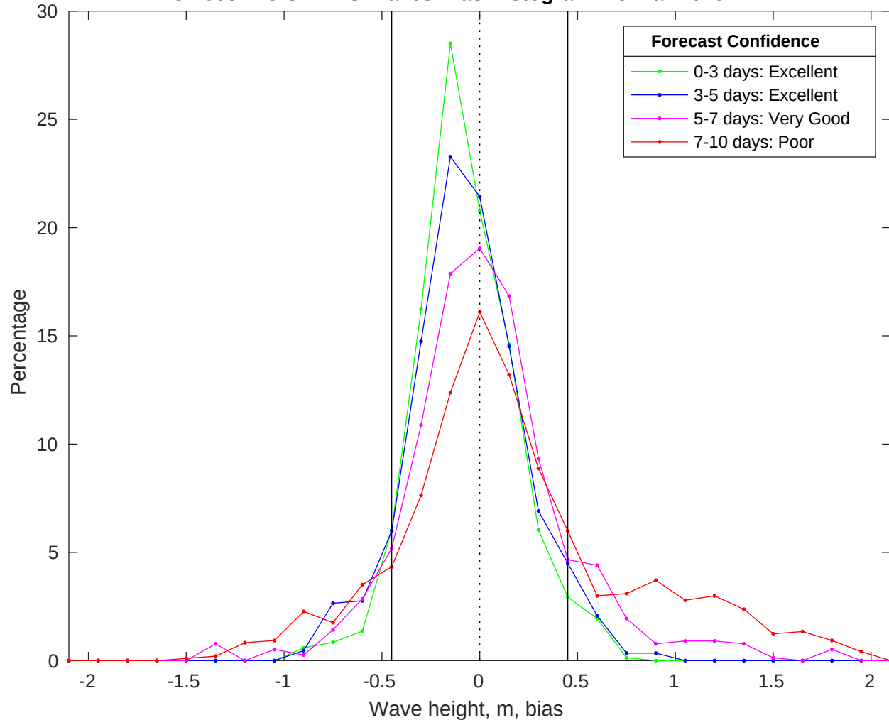
NDBC 46054 vs CMEMS Waves Bias Histogram: 25-Mar-2025
