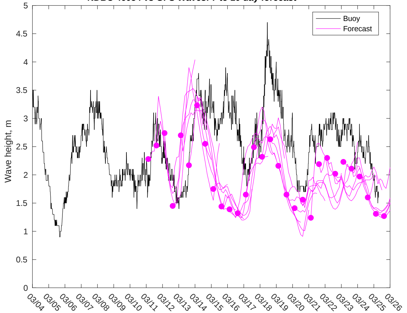
NDBC 46054 vs GFS Waves: 7 to 10 day forecast
