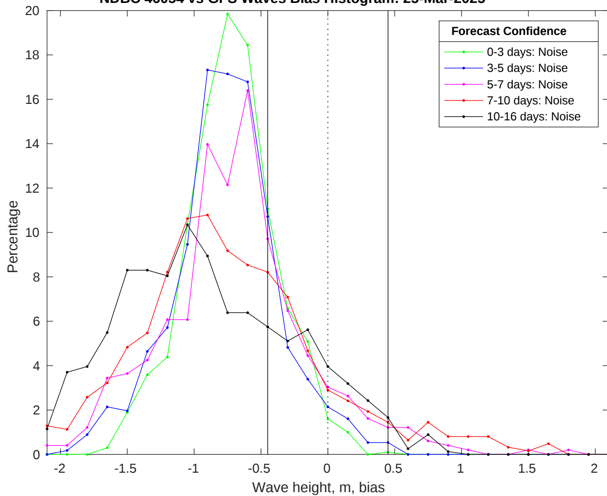
NDBC 46054 vs GFS Waves Bias Histogram: 25-Mar-2025
