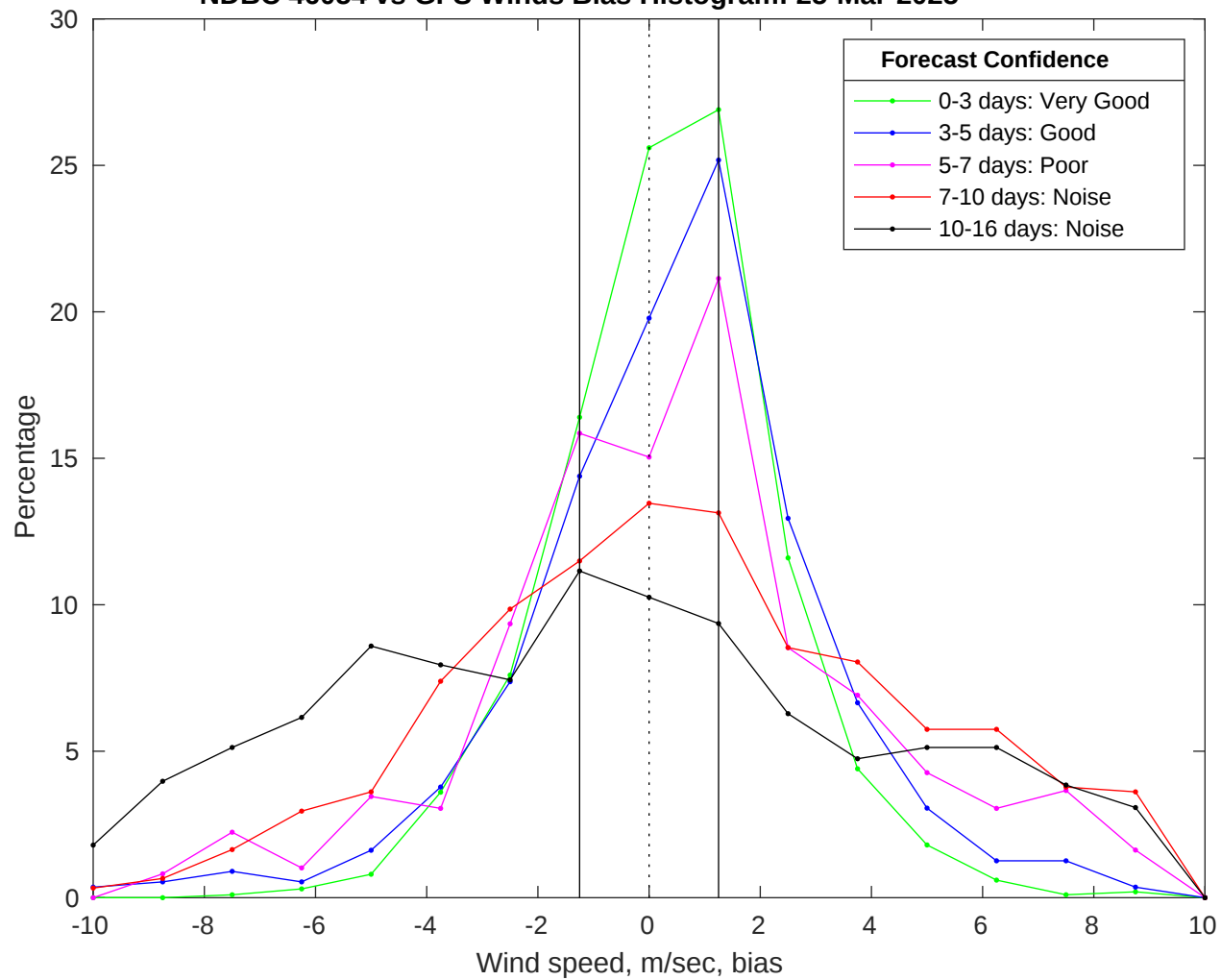
NDBC 46054 vs GFS Winds Bias Histogram: 25-Mar-2025
