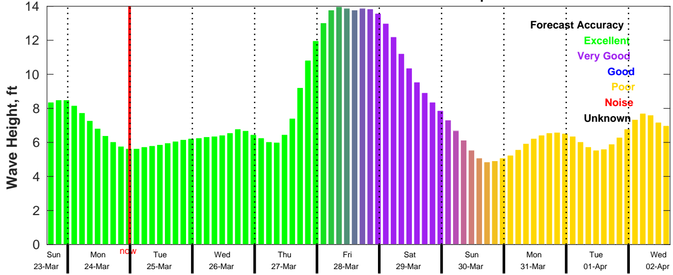
CMEMS Wave Forecast for NDBC 46054 from 23-Mar-2025 16:00:00 to 02-Apr-2025 16:00:00
