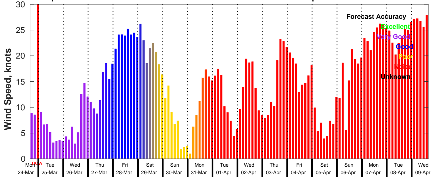
GFS Wind Speed Forecast for NDBC 46054 from 24-Mar-2025 16:00:00 to 09-Apr-2025 16:00:00
