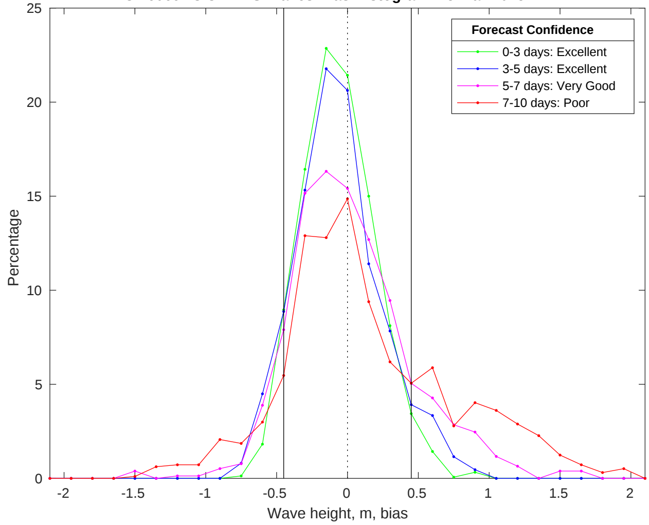
NDBC 46069 vs CMEMS Waves Bias Histogram: 25-Mar-2025
