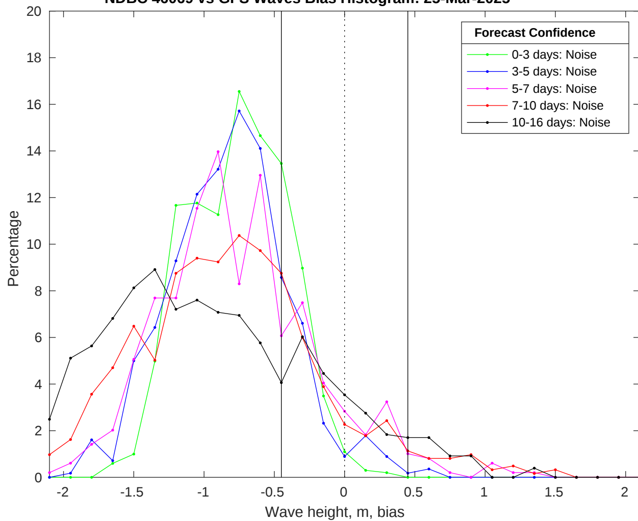
NDBC 46069 vs GFS Waves Bias Histogram: 25-Mar-2025
