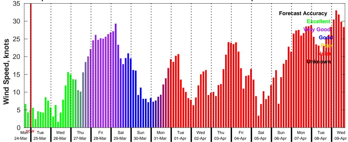
GFS Wind Speed Forecast for NDBC 46069 from 24-Mar-2025 16:00:00 to 09-Apr-2025 16:00:00
