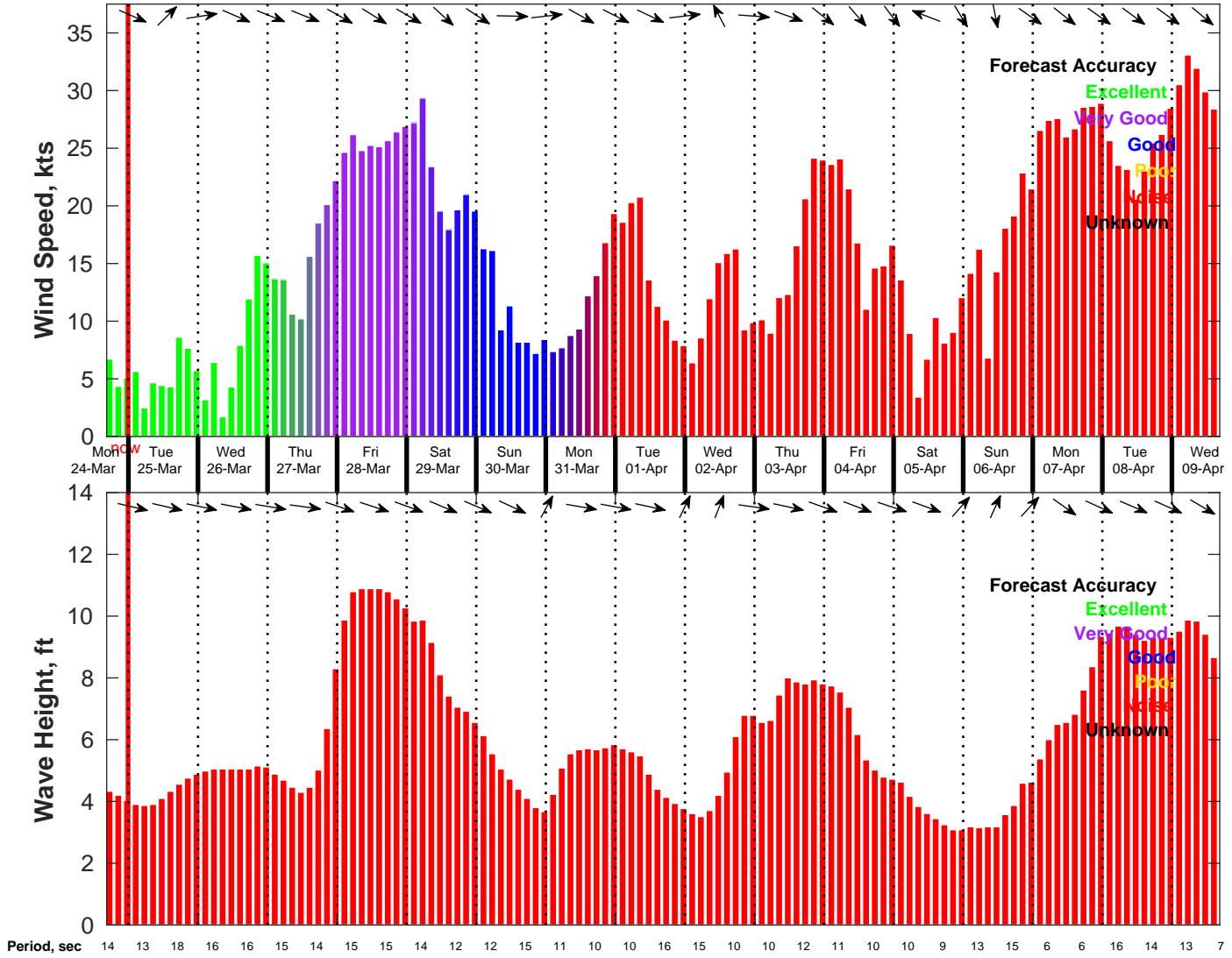
Wind & Wave Forecast for NDBC 46069 from 24-Mar-2025 16:00:00 to 09-Apr-2025 16:00:00
