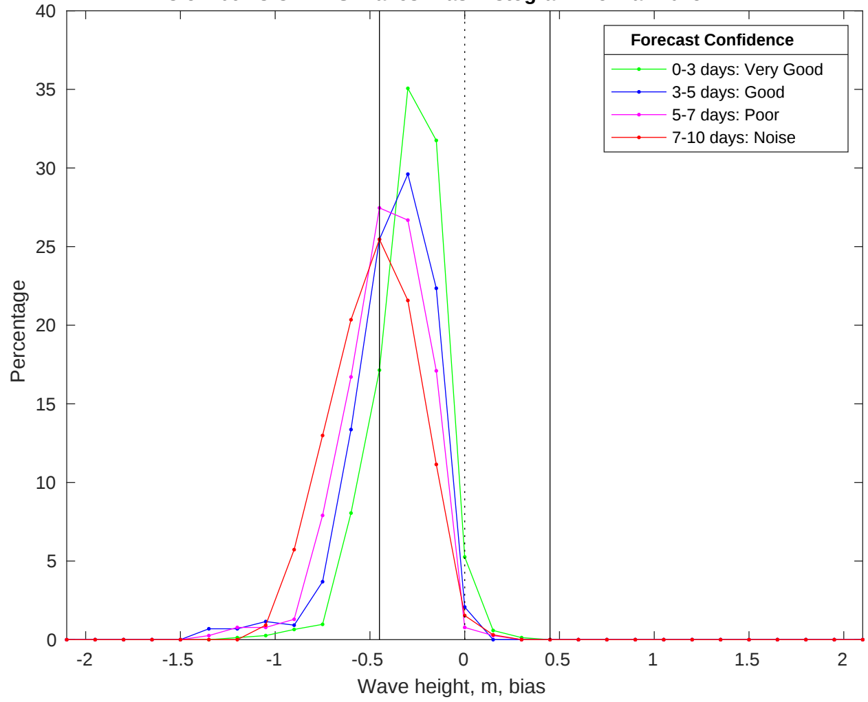
NDBC 51209 vs CMEMS Waves Bias Histogram: 25-Mar-2025
