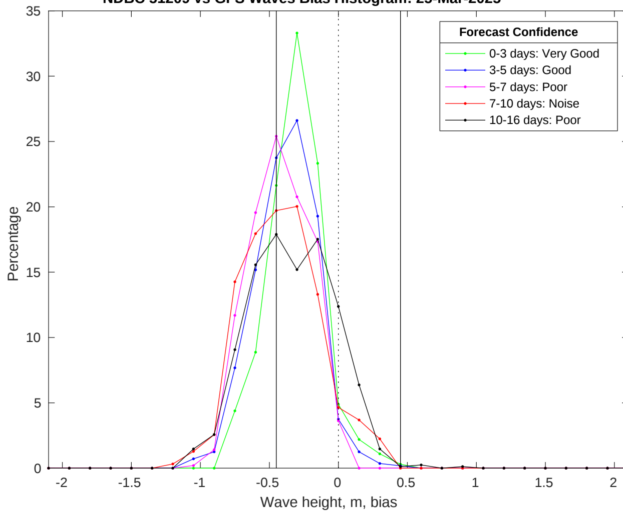
NDBC 51209 vs GFS Waves Bias Histogram: 25-Mar-2025
