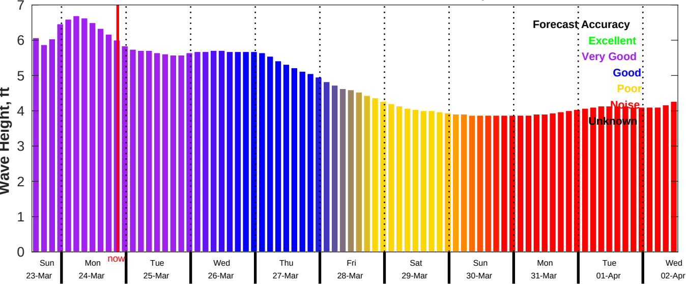
CMEMS Wave Forecast for NDBC 51209 from 23-Mar-2025 13:00:00 to 02-Apr-2025 13:00:00
