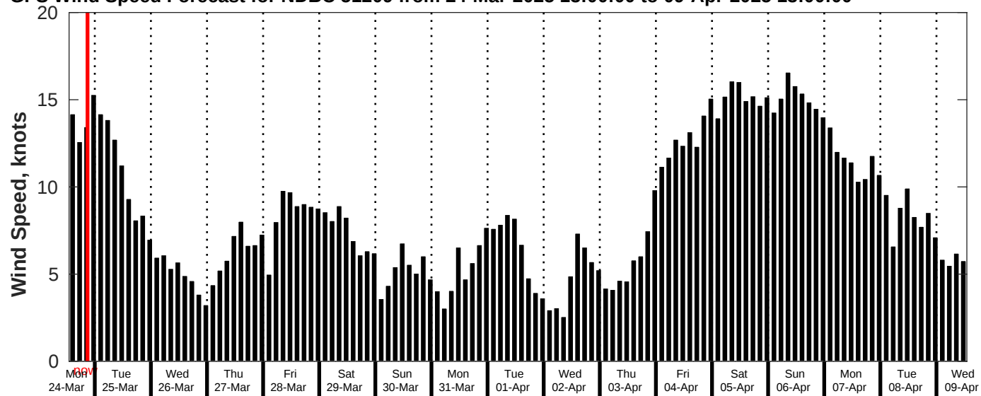
GFS Wind Speed Forecast for NDBC 51209 from 24-Mar-2025 13:00:00 to 09-Apr-2025 13:00:00
