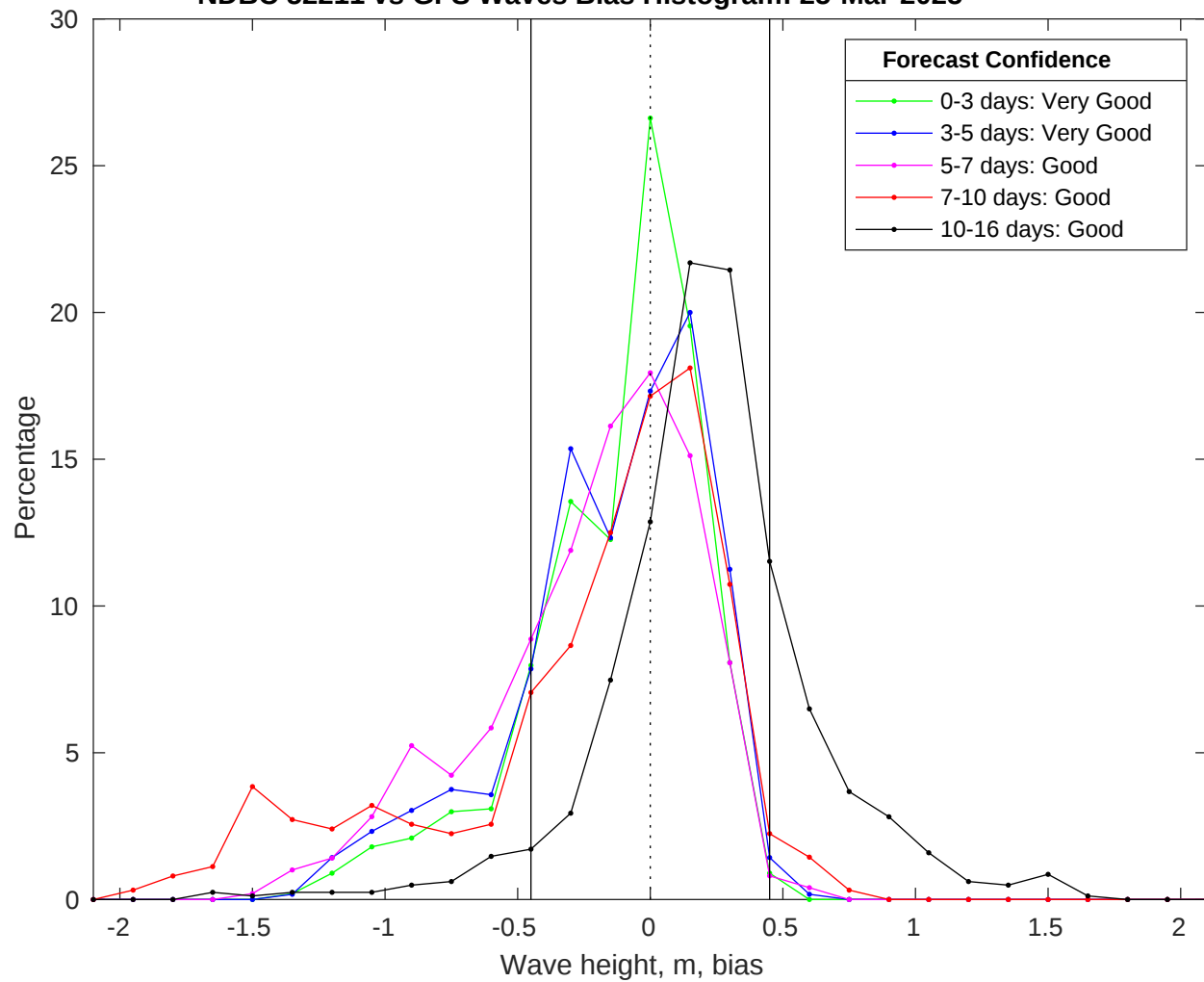
NDBC 52211 vs GFS Waves Bias Histogram: 25-Mar-2025
