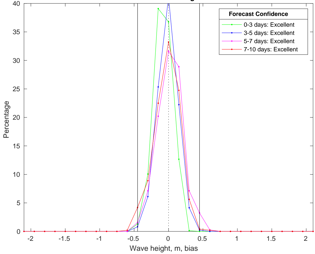
NDBC 52212 vs CMEMS Waves Bias Histogram: 25-Mar-2025
