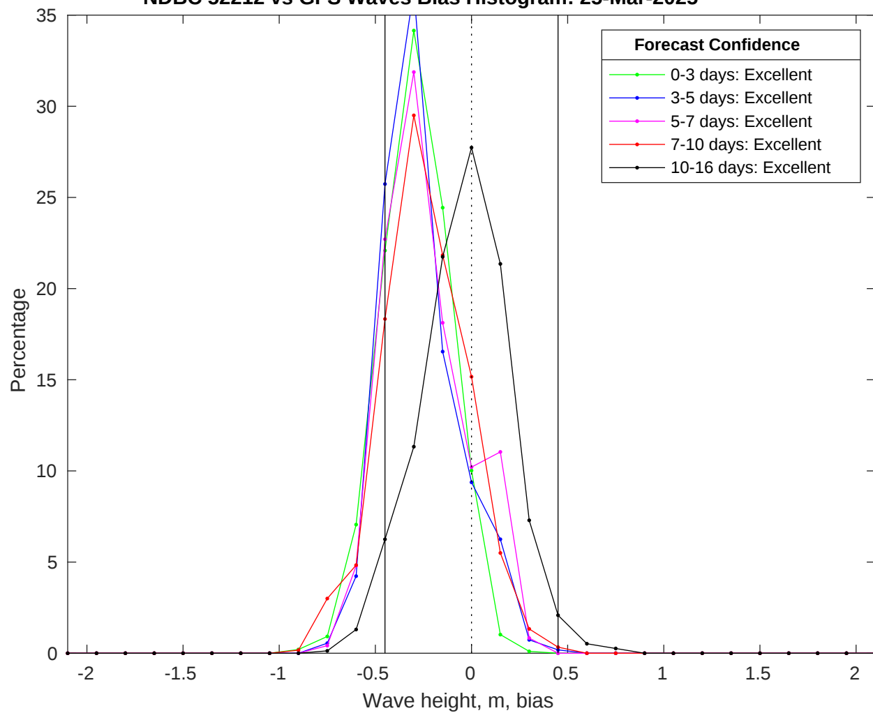
NDBC 52212 vs GFS Waves Bias Histogram: 25-Mar-2025
