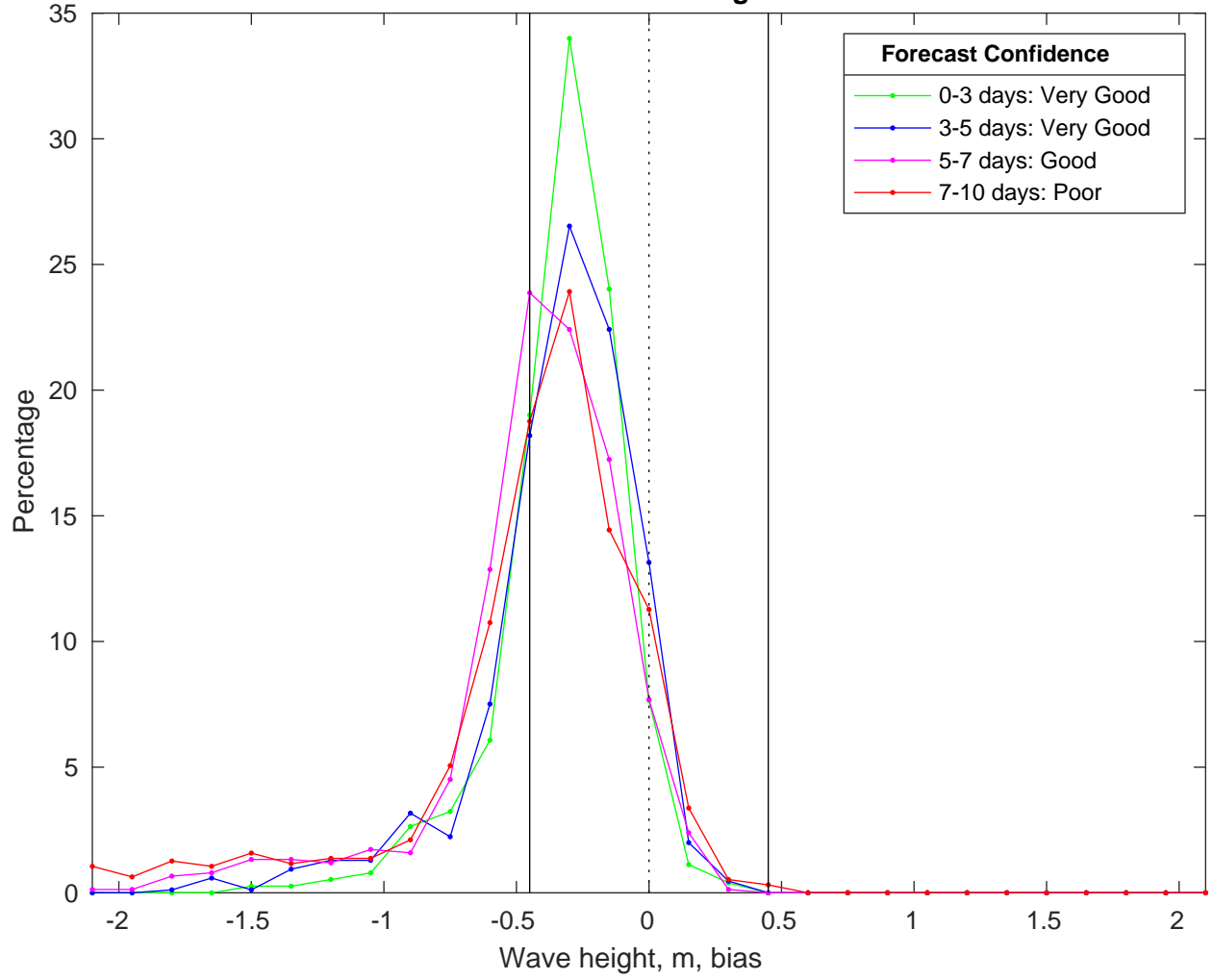
NDBC 52213 vs CMEMS Waves Bias Histogram: 25-Mar-2025
