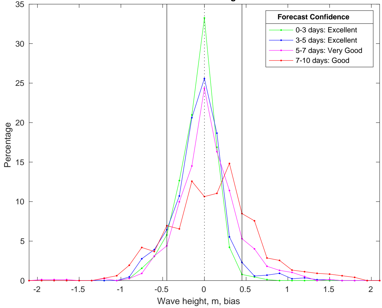
NDBC 41004 vs CMEMS Waves Bias Histogram: 26-Mar-2025
