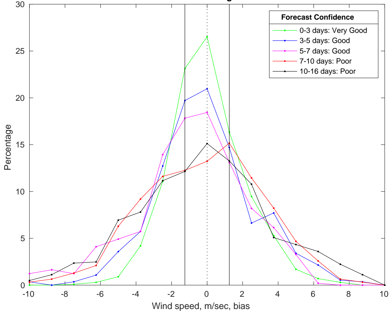
NDBC 41004 vs GFS Winds Bias Histogram: 26-Mar-2025
